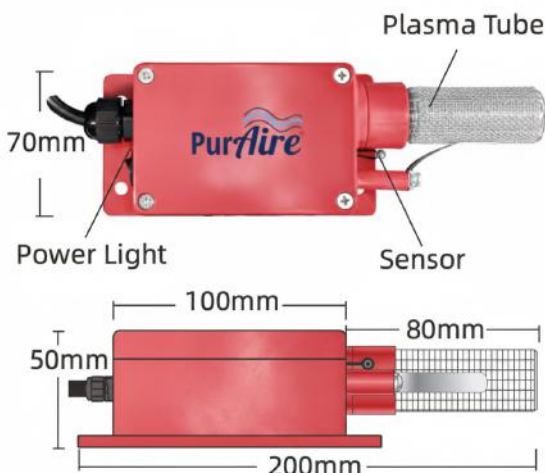
SG-Mini-5A Dimensions
