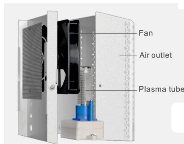
Exploded View
